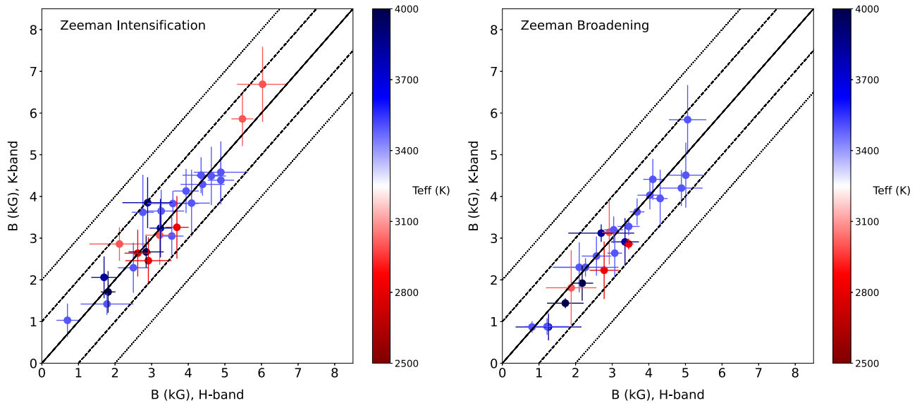
Figure 8. Comparison between the measured magnetic field strengths from IGRINS H - and K -band spectra. The left panel shows the measurements using the Zeeman intensification method and the right panel shows the measurements using the Zeeman broadening method. In both panels, solid black lines mark the 1-to-1 relations, and dashed and dotted lines mark 1 and 2 kG offsets. Different colored circles represent T_{\text{eff}} for the individual stars.
