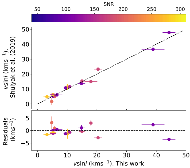
Figure 2. Comparison of v\sin i measurements from this work to values from Shulyak et al. (2019). The bottom panel shows the difference between Shulyak et al. (2019) and this work.
