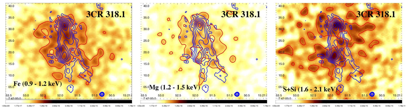
Figure 3. Narrowband Chandra flux images in the 0.9–1.2 keV (left), 1.2–1.5 keV (center), and 1.6–2.1 keV (right) energy bands to show Fe, Mg, and S+Si X-ray emissions with [N II] \lambda 6584 contours overlaid. Chandra images were smoothed with a Gaussian kernel of 2'' . [N II] \lambda 6584 emission line contours are the same as in Figure 2. X-ray emission due to Mg seems to trace the [N II] \lambda 6584 morphology the best. X-ray fluxes along the filament (regions sw4 and sw14) are F_{\text{Fe}} = 2.9^{+0.2}_{-0.3} \times 10^{-14} \text{ erg s}^{-1} \text{ cm}^{-2} in the Fe band, F_{\text{Mg}} = 1.9^{+0.1}_{-0.1} \times 10^{-14} \text{ erg s}^{-1} \text{ cm}^{-2} in the Mg band, and F_{\text{S+Si}} = 2.3^{+0.1}_{-0.2} \times 10^{-14} \text{ erg s}^{-1} \text{ cm}^{-2} in the S+Si band.
