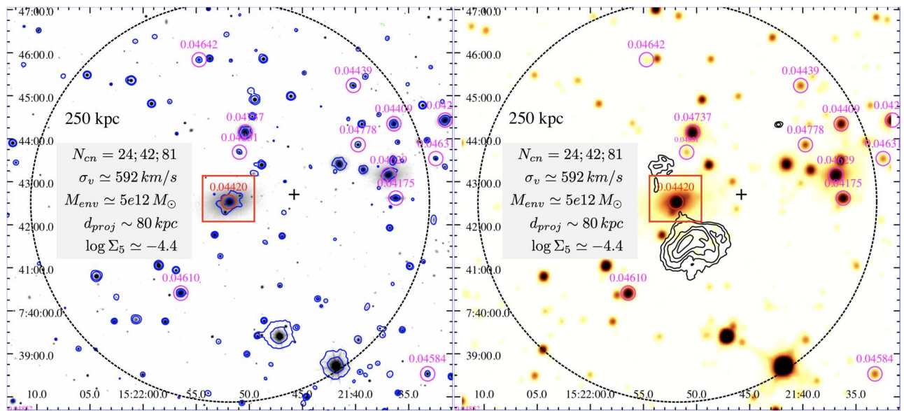
Figure 1. r -band SDSS image with SWIFT UV contours at 2600 \text{ \AA} overlaid in blue (left) and 3.4 \mu\text{m} WISE image with 328 MHz VLA radio contours overlaid in black (right), showing 3CR 318.1 at the center and other sources in the field. The red squares show MUSE field of view. Radio contours were drawn at 5, 10, 20, 40, and 80 times the rms level of the background in the radio map (beam size of 5''/4 ). Sources in the field with known spectroscopic redshifts are marked in magenta. Ambient parameters, shown in both panels, were derived according to Massaro et al. (2019, 2020, 2020). N_{\text{cn}} is the number of cosmological neighbors within a radius of 500 kpc, 1 Mpc, and 2 Mpc, respectively; \sigma_v is the velocity dispersion of the cosmological neighbors; M_{\text{env}} is the environmental mass (i.e., galaxies, IGM and dark matter) estimated from the velocity dispersion; d_{\text{proj}} is the projected distance between the central radio galaxy and the centroid of the position of the cosmological neighbors within 2 Mpc (marked by the black cross); and \Sigma_5 is the cosmological parameter used to trace the dark matter halo density (see Sabater et al. 2013; Worpel et al. 2013). SWIFT-UVOT data were reduced according to the standard procedure (see Massaro et al. 2008a, 2008b for more details).
