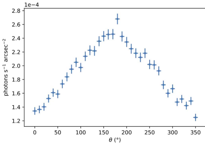
Figure 5. 0.5–3 keV, exposure-corrected, X-ray surface brightness profile with azimuthal bins of 10^\circ centered on the core of 3CR 318.1. The bins were chosen so that the bin at 180^\circ is the one containing the [\text{N II}]\lambda 6584 filament. Background level is two orders of magnitude below the filament emission. The increase of surface brightness corresponds to [\text{N II}]\lambda 6584 .
