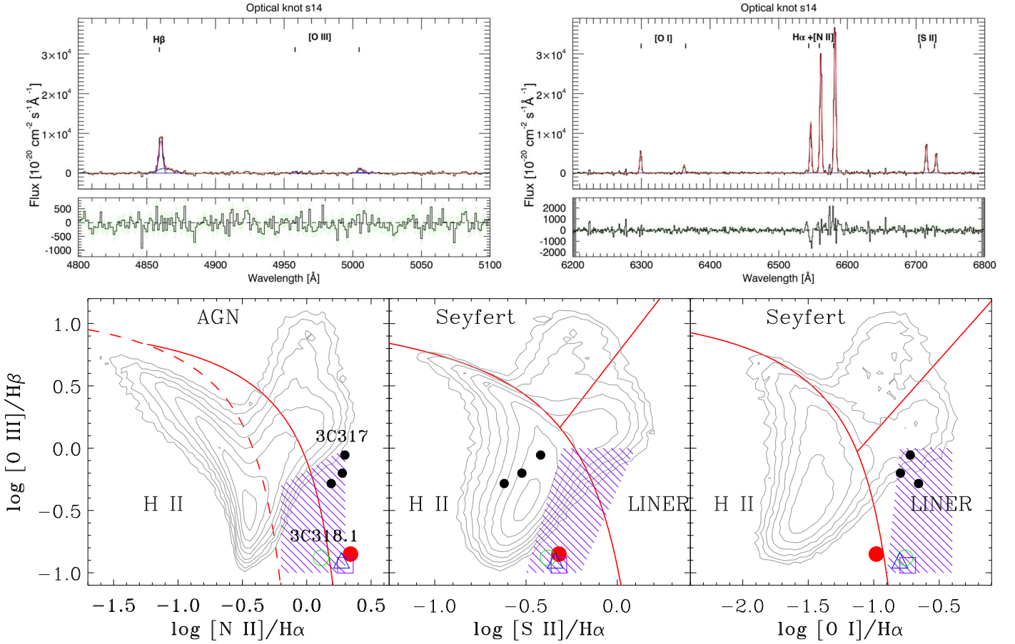
Figure 4. Top: MUSE spectrum (black histograms) of region s14; see Figure 2, in rest frame, shown as an example. We show in red the Gaussian fit of the emission lines (top panels) and the residuals (bottom panels). Bottom: location of 3CR 318.1 regions “core,” s14, sw4, and sw14 (red filled circle, green circle, blue triangle, and magenta square, respectively) in the Baldwin, Phillips & Telervich (BPT) diagnostic diagrams. The red solid curves represent the Kewley et al. (2001) theoretical upper bound for pure star formation, the red straight line shows the Kewley et al. (2006) separation between AGN and LINERs, while the dashed red curve in the [N II] \lambda 6584 BPT is the Kauffmann et al. (2003) empirical classification separating star-forming galaxies and AGN. Contours represent the isodensities of all SDSS/DR7 emission line galaxies (Capetti & Baldi 2011). The three black dots mark the location of the filaments in 3CR 317, the central galaxy of A2052, also observed as part of the MURALES survey (see Balmaverde et al. 2018). Purple dashed regions mark the location of filaments in other cool core galaxy clusters as measured by McDonald et al. (2012).
