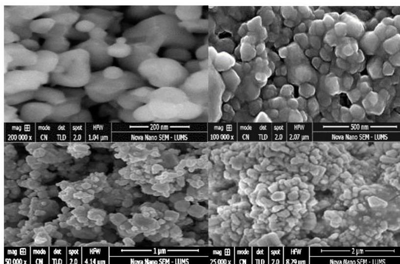
Fig. 2. SEM pictures of ZnO nanoparticles
