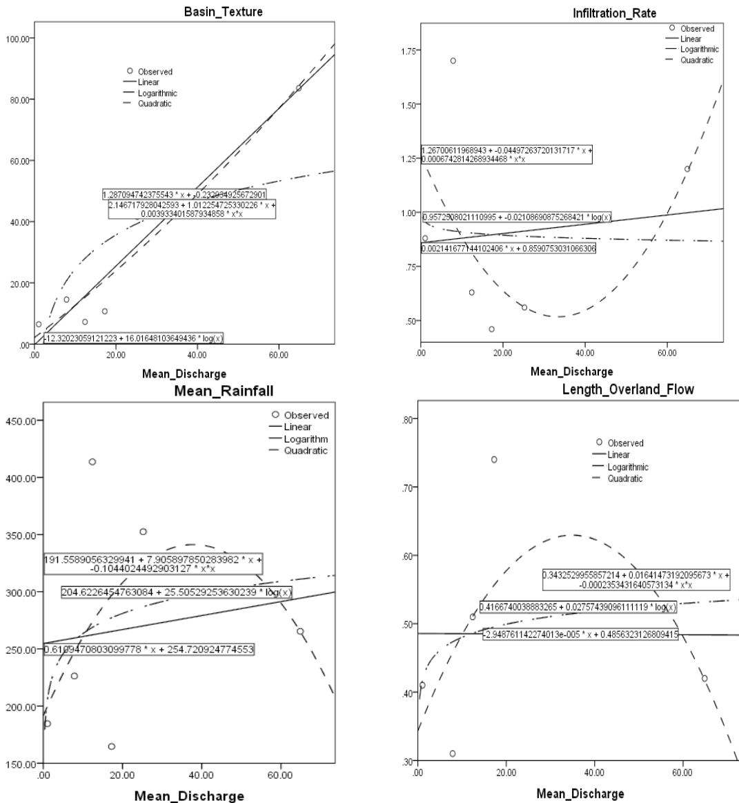
Fig. 2. The relationships between mean discharge and the four independent variables
