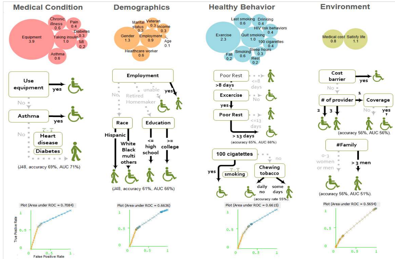
Fig. 4. Infographics of correlation models for disability among post-stroke patients generated using C4.5 (J48) algorithm using Weka software
